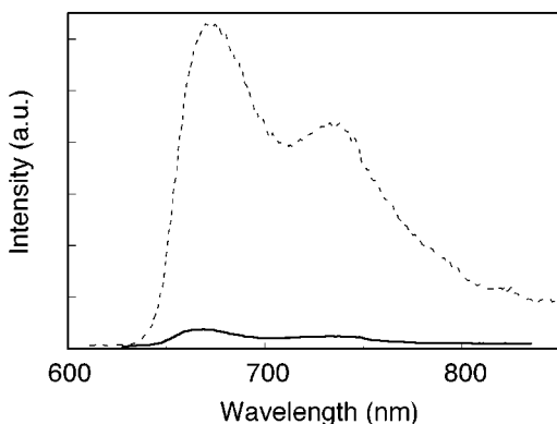
Figure 2. Fluorescence spectra of Por-4T (dashed line) and Por-4T-C60 (solid line) in benzonitrile with excitation at 558 nm.
