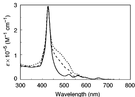
Figure 1. Electronic absorption spectra of Por-4T-C60 (solid line), Por-8T-C60 (dashed line), and Por-12T-C60 (dotted line) in benzonitrile.
