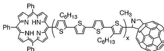
Por-nT-C60 ( x = 1-3 )
